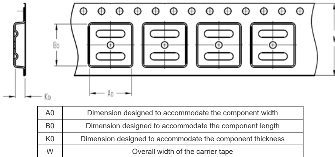
Figure 26 Specification Drawing of Reel Packaging
